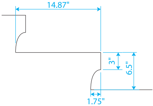
York Steps - Stair Detail B
