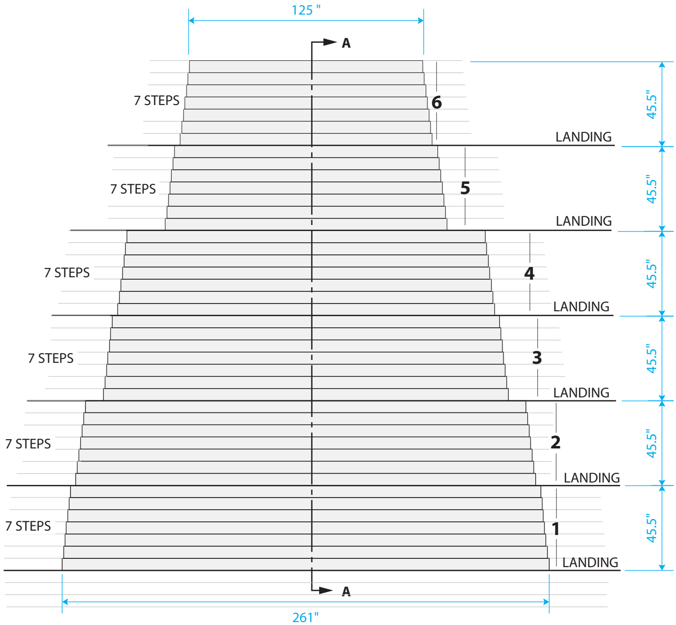
York Steps - Elevation
