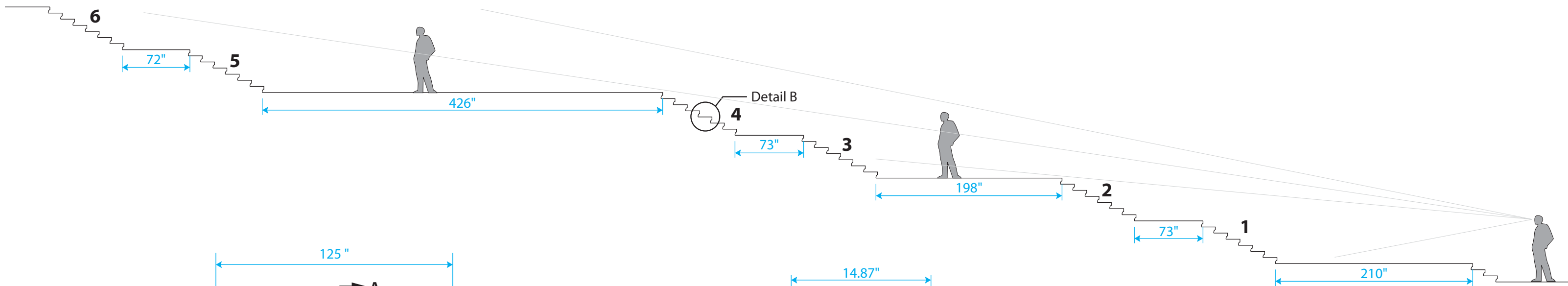
York Steps - Section AA
